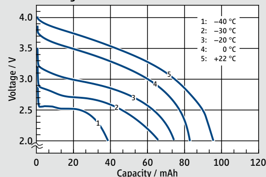
Discharge Curve at 500 mA
