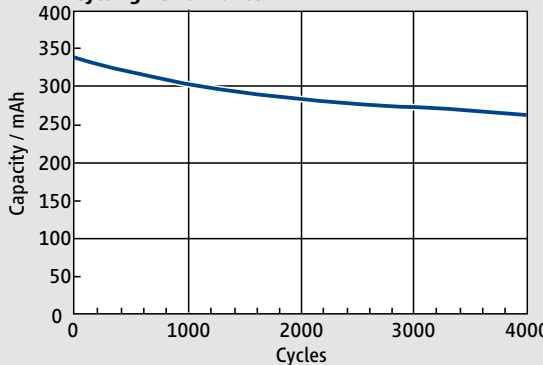
Cycling Performance
