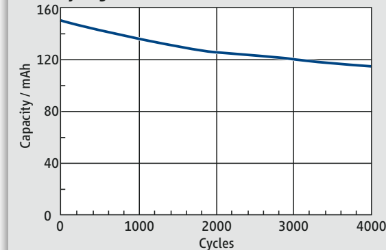
Cycling Performance
