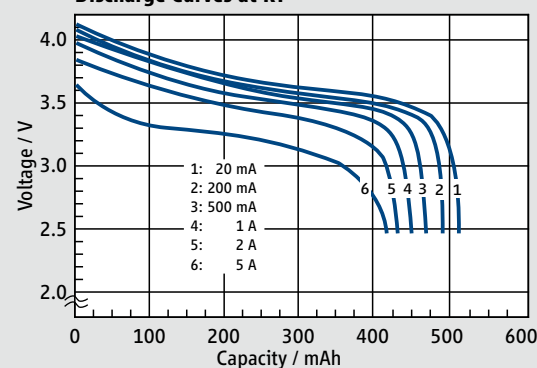
Discharge Curves at RT
