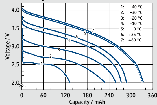
Discharge Curve at 2 A
