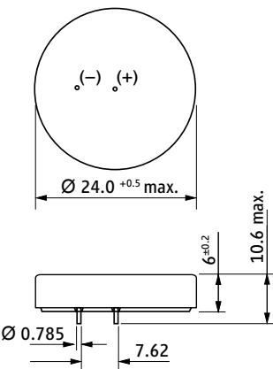
TL-2450 (with insolation disc)
