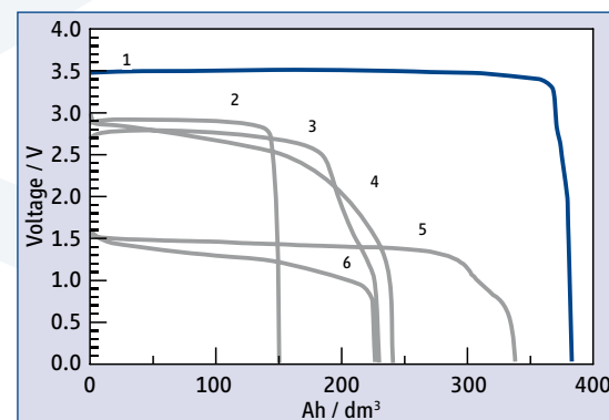
Figure 2: Comparison of different battery systems. The curves represent typical best values of commercial cylindrical cells when discharged at +25^{\circ}\text{C} at the 1000 hour rate. The area under the curves corresponds to the energy density listed below.
