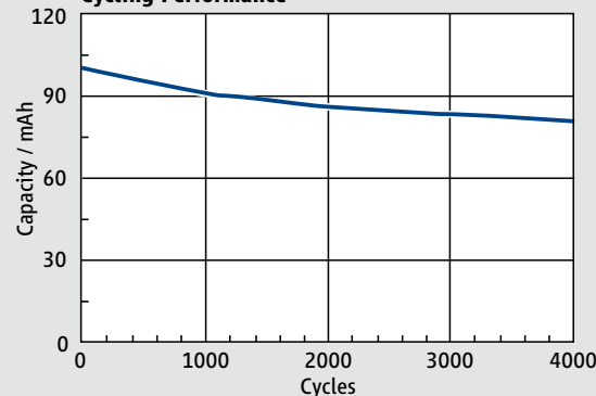
Cycling Performance
