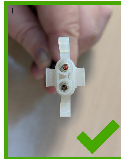
(G - J) Multiple angles of the connector are needed to help determine the correct connector. (J) A clear photo of how the wires, from the battery, fit into the connector is important to ensure correct polarity.
